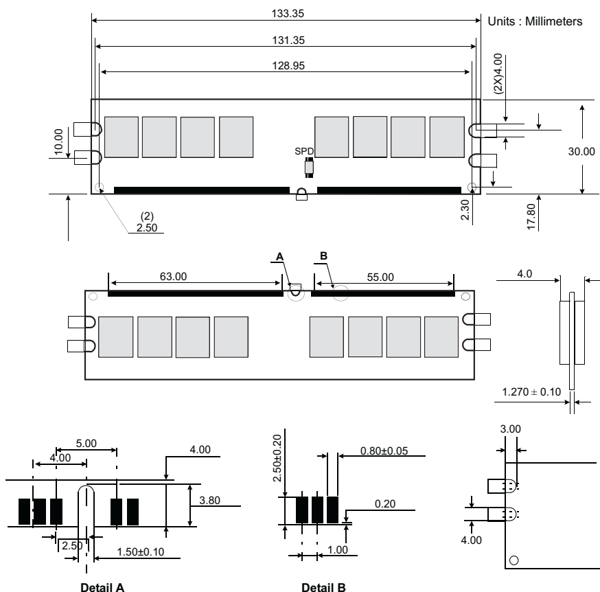
Figure 1: KVR667D2N5K2/2G 240-Pin DIMM Kit
